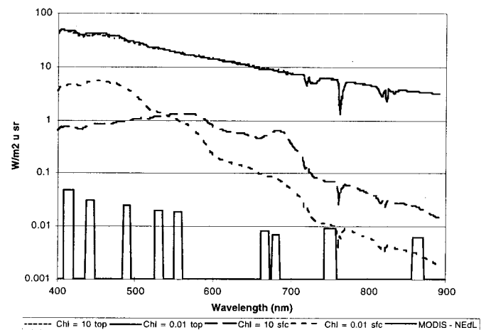
Fig. 1. Upwelling radiance at the TOA and at the ocean surface for extremely low- and very high-oceanic chlorophyll a concentrations. (four lines from top to bottom on left are TOA: 0.01 mg/m 3 , TOA: 10 mg/m 3 , surface: 0.01 mg/m 3 , and surface: 10 mg/m 3 ). Model radiances simulate a nadir view at 60° solar zenith angle, or a clear atmosphere with an aerosol optical depth at 670 nm of 0.2, Angstrom exponent of 0.5, 5-mm precipitable water, and 0.35-cm ozone. Measured values of Noise-Equivalent Delta Radiance (NEDL) for MODIS bands 8–16 are shown as bars.
