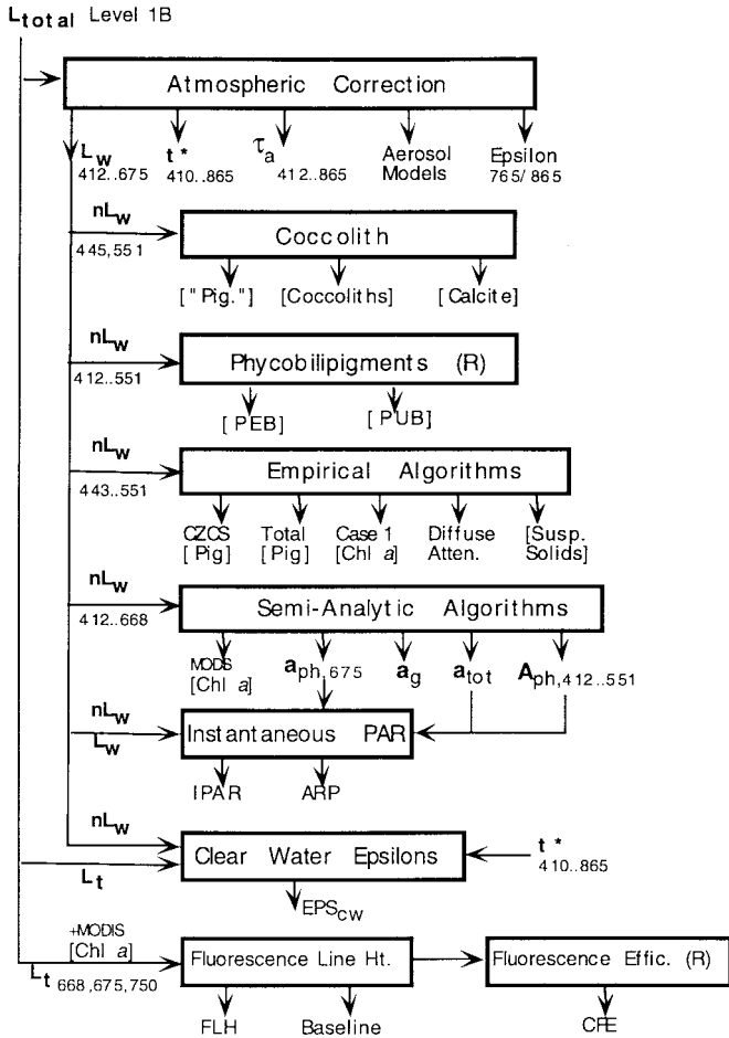
Fig. 3. MODIS Ocean Color Level 2 Simplified Algorithm Flow diagram. Geophysical products are at arrow terminations.
